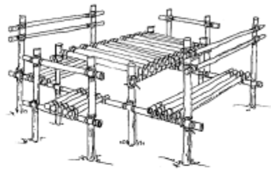
Camp Table with Bench and Seat
