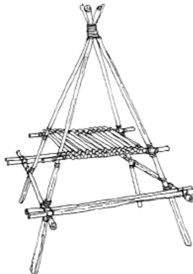
Camp Table with Seats
