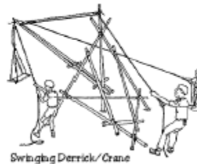
Swinging Derrick/ Crane
