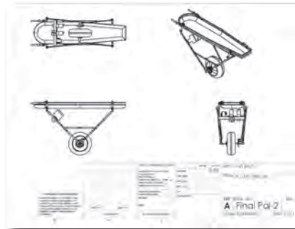
A 2D drawing of second PAL prototype
