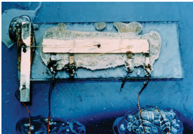
Jack Kilby invented the integrated circuit at Texas Instruments in 1958. Composed of only a transistor and other components on a slice of germanium, Kilby's invention, \frac{7}{16} by \frac{1}{16} inches in size, revolutionized the electronics industry and our lives.
