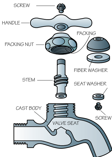
Compression faucet
