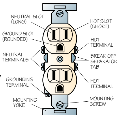
Grounded three-slot 120-volt duplex outlet
