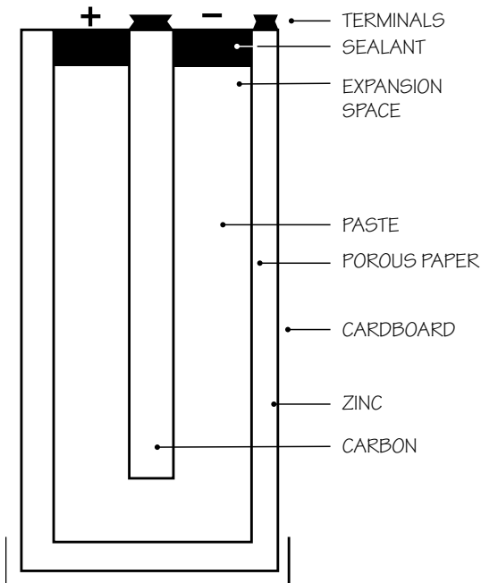
A dry cell is designed for on-and-off use.
